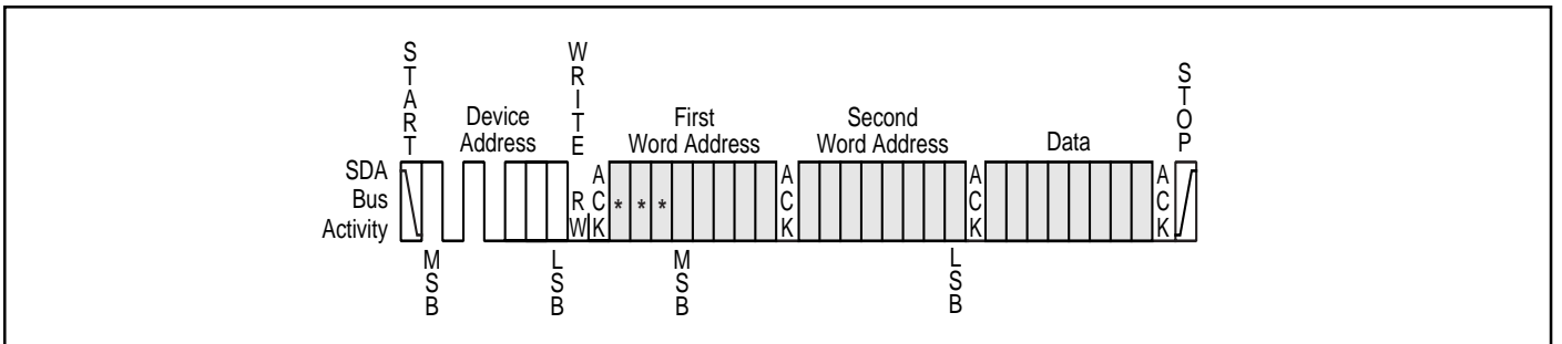
Figure 6. Byte Write
