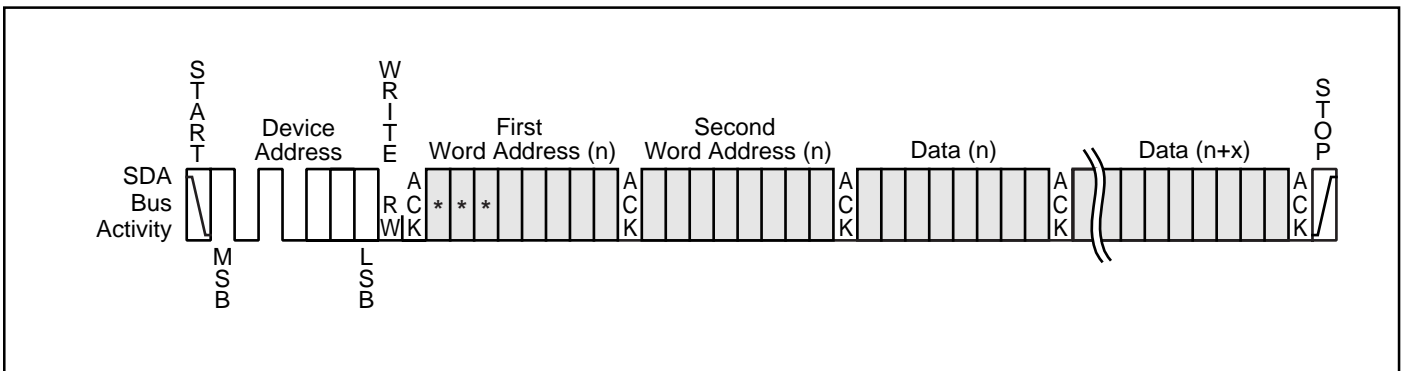
Figure 7. Page Write
